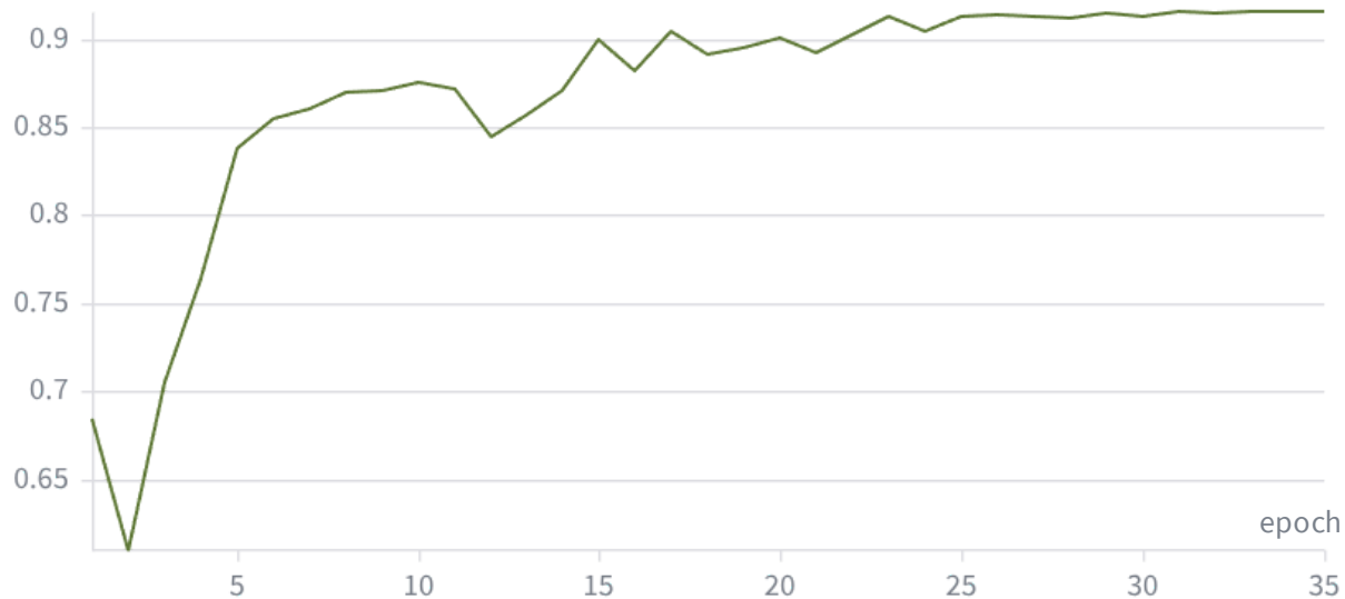
val_dice_TC
